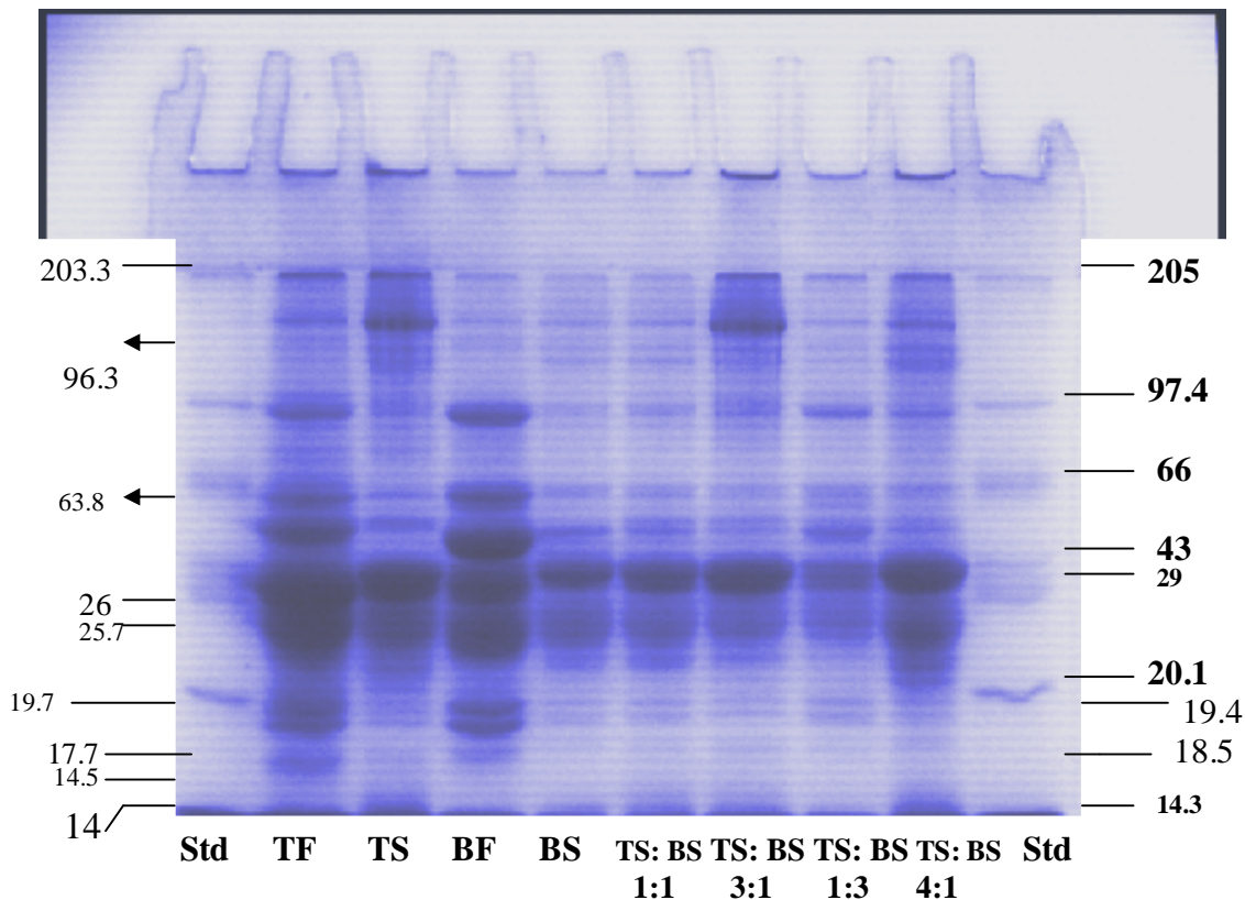
Figure1: SDS-PAGE pattern of water soluble proteins of intact fillets, surimi and surimi mixtures of threadfin bream and bulls-eye. The numerical values are molecular weights (kD) of the protein bands. TF: threadfin bream fillet; TS: threadfin bream surimi; BF:bull's-eye fillet; BS:bull's-eye surimi.
